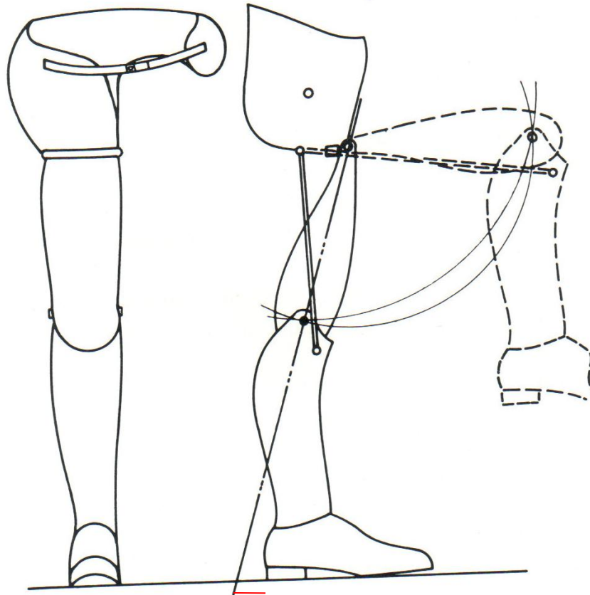
Fig. 26-6. Alignment principle of Canadian hip disarticulation prosthesis.
